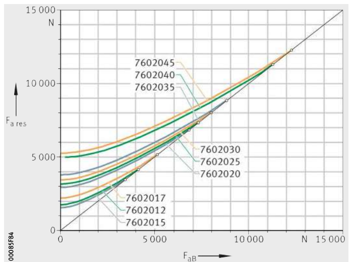
Figure 32 Resultant bearing load for 7602012 to 7602045
