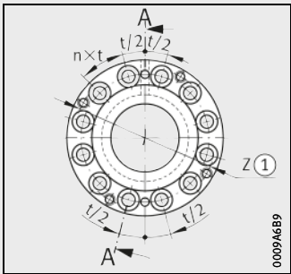
Hole pattern
