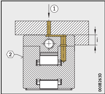
Oil feed
