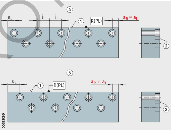
Figure 10 Hole patterns of guideways with offset rows of holes
