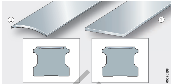
Figure 3 Guideway covering strip
