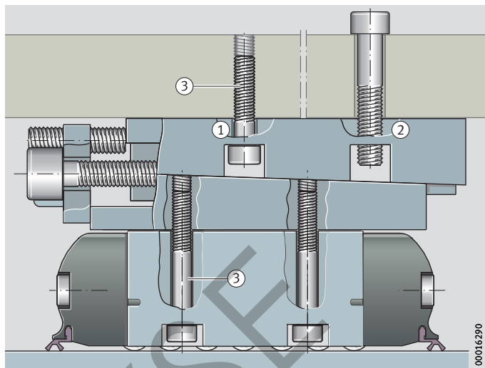
Figure 17 Location of linear roller bearing with adjusting gib assembly
