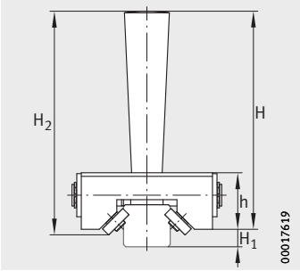
ERVS...-B Front view
