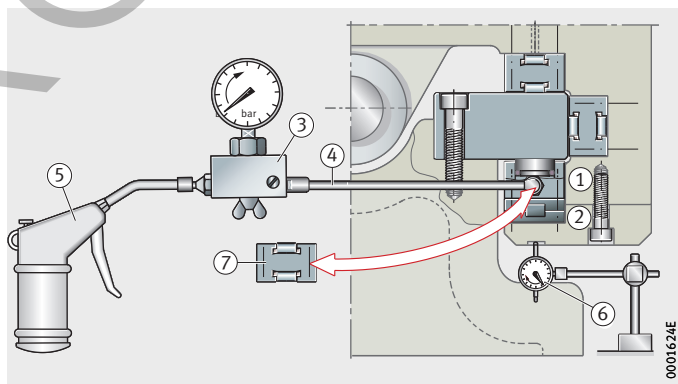
Figure 4 Measuring the preload dimension using the setting device
