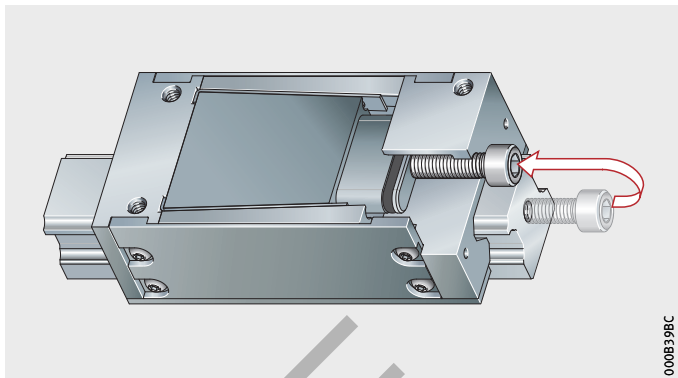
Figure 10 Braking and clamping element on support rail
