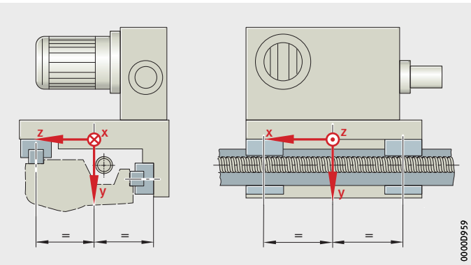
Figure 4 Defining the table co-ordinate system
