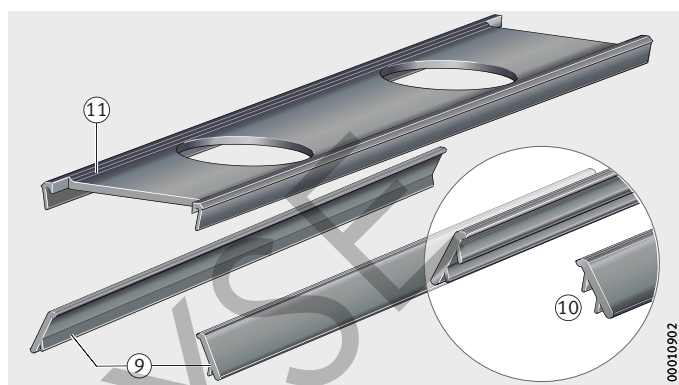
Figure 5 Sealing strips KIT.RWU..-910, -920, -930
