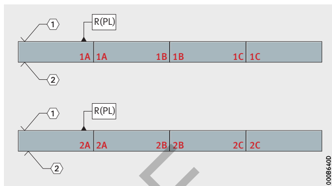
Figure 9 Marking of multi-piece guideways
