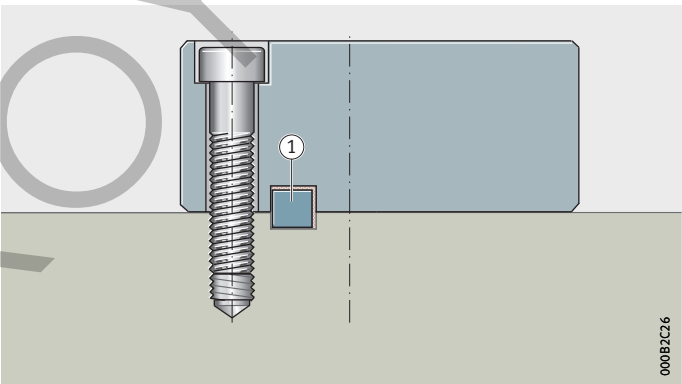
Figure 5 Guideway with longitudinal slot and square steel bar
