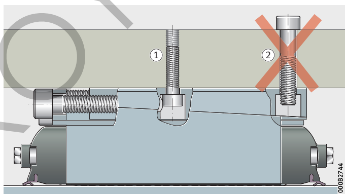
Figure 18 Location of linear roller bearing with integrated adjusting gib assembly
