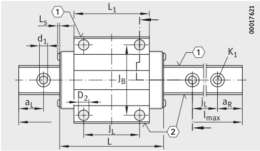
KUE...-B-E View X rotated 90°
