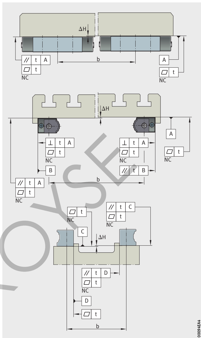
Figure 5 Tolerances of mounting surfaces and parallelism of mounted guideways and linear recirculating ball bearing units
