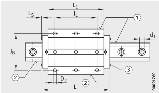
RUE100-E-L
