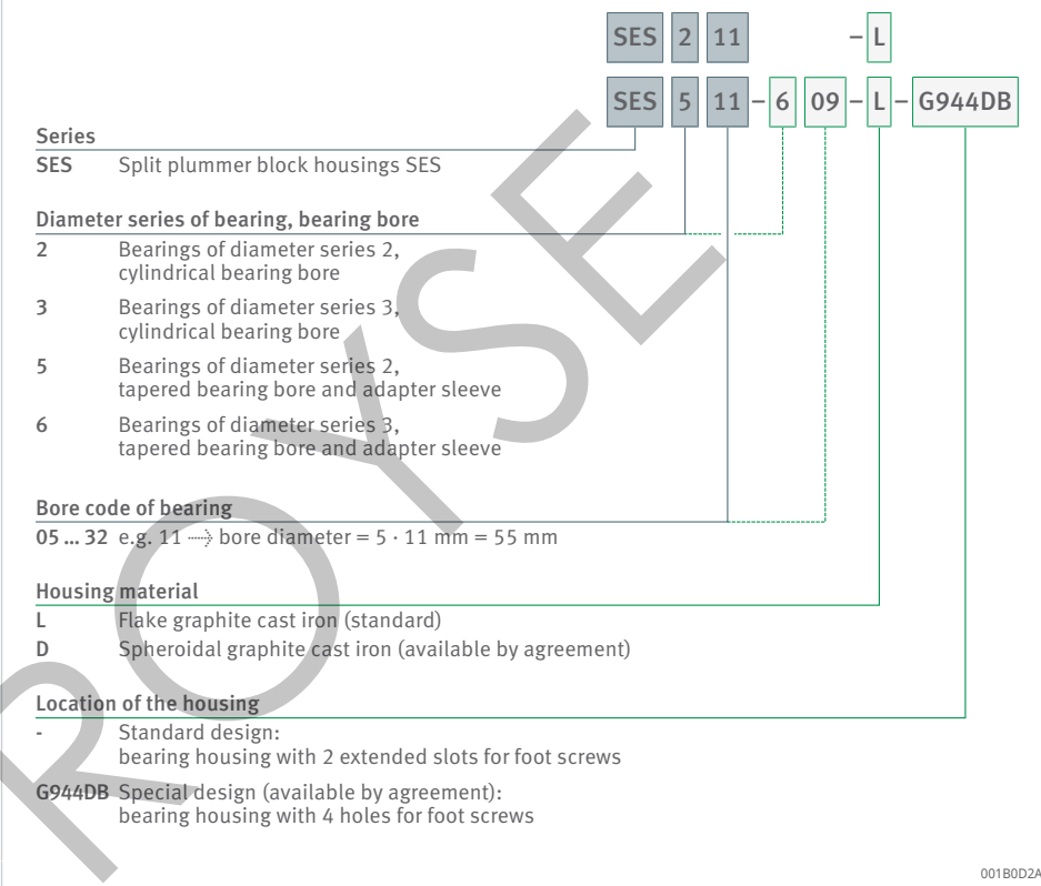
19 Designation structure of plummer block housings SES, examples
