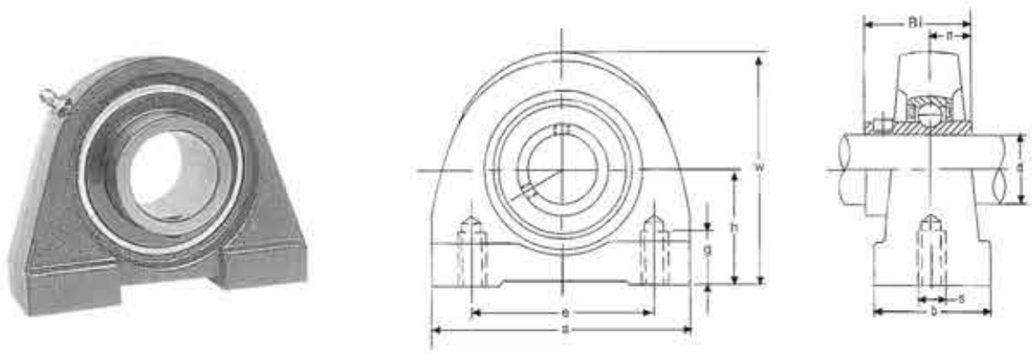
UCPW200 Series
