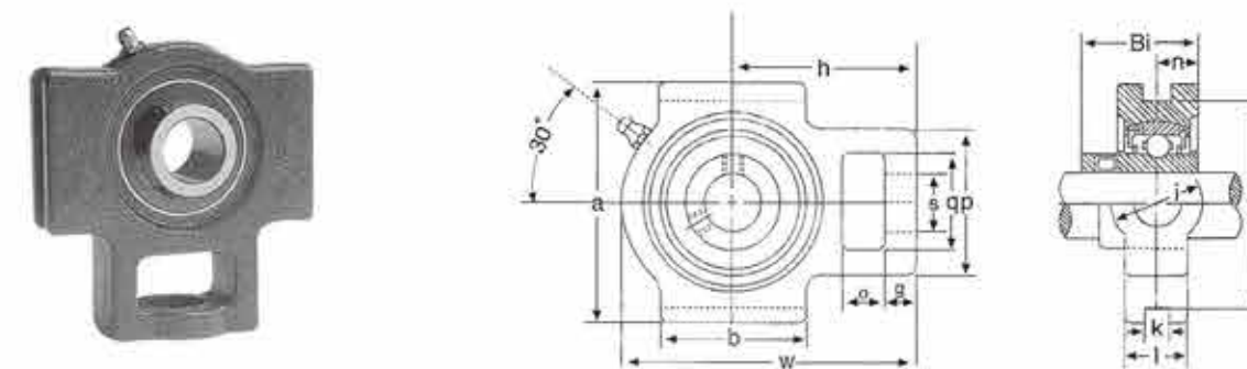
UCT200 Series
