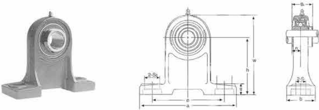
UCPH200 Series
