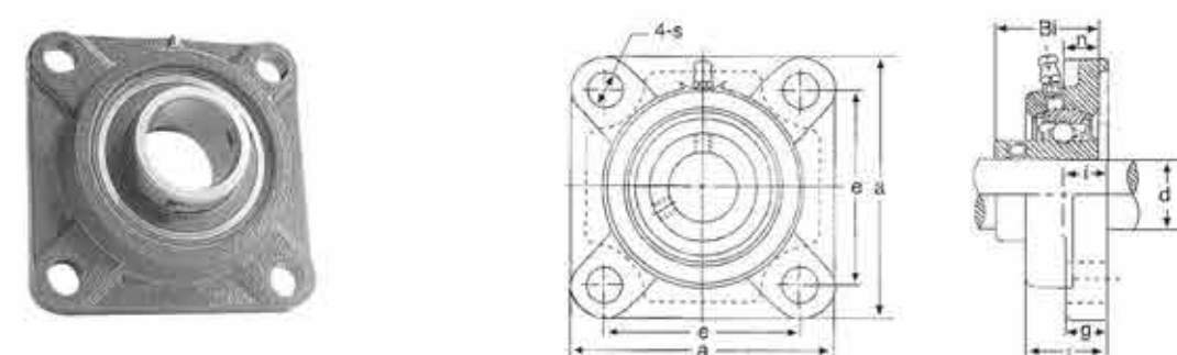
UCF200 Series
