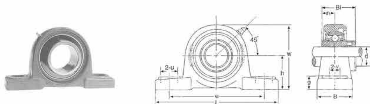
UCP300 Series
