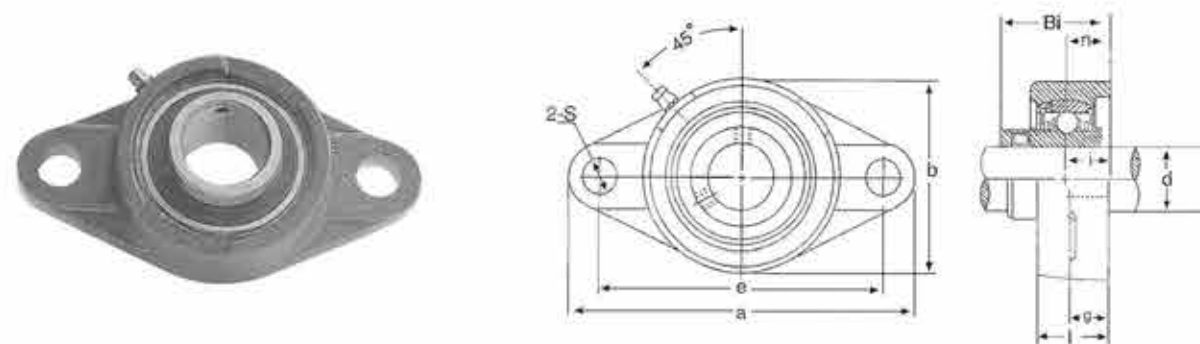
UCFL300 Series
