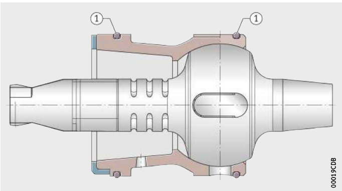
Figure 12 Gear lever bearing arrangement
