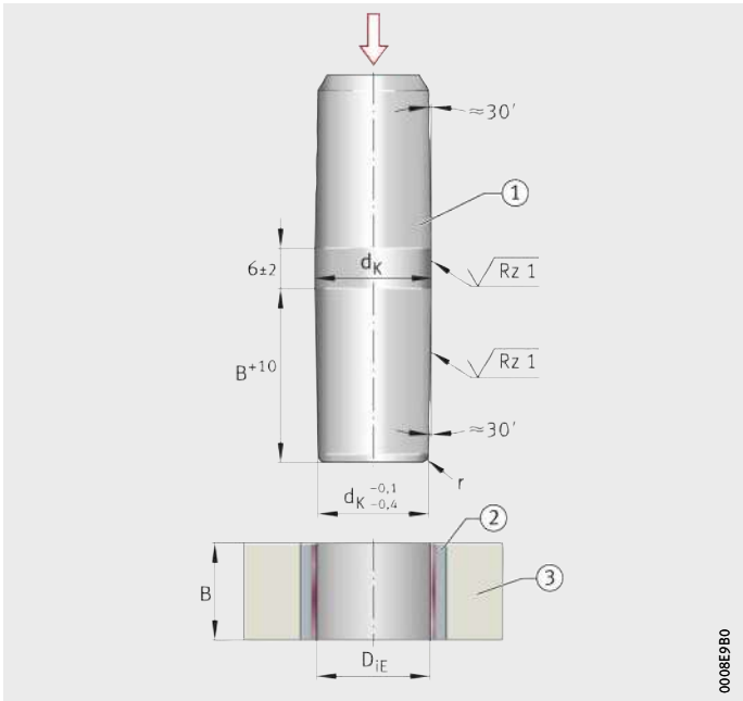
Figure 7 Sizing of plain bearing bush
