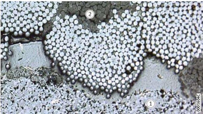
Figure 1 Microsection of a ELGOTEX filament wound bush
