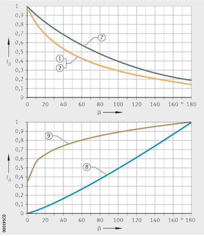
Figure 26 Correction factor for swivel and oscillation angle
