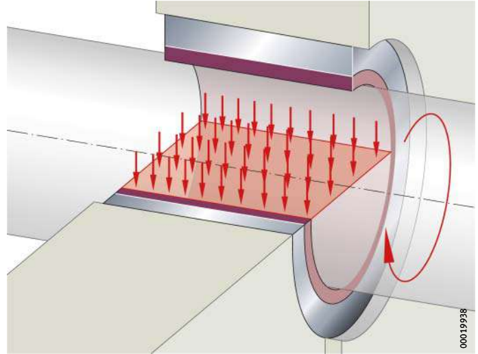
Figure 7 Projected area of a bush
