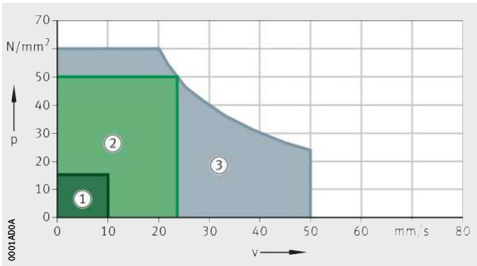
Figure 2 pv diagram
