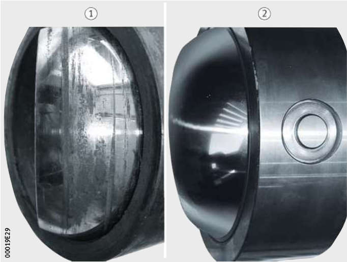
① Before reconditioning ② After reconditioning Figure 1 Spherical plain bearing before and after reconditioning
