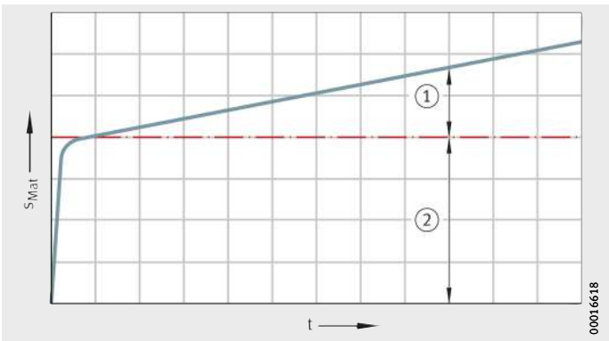
Figure 5 Typical operating behaviour during operating life
