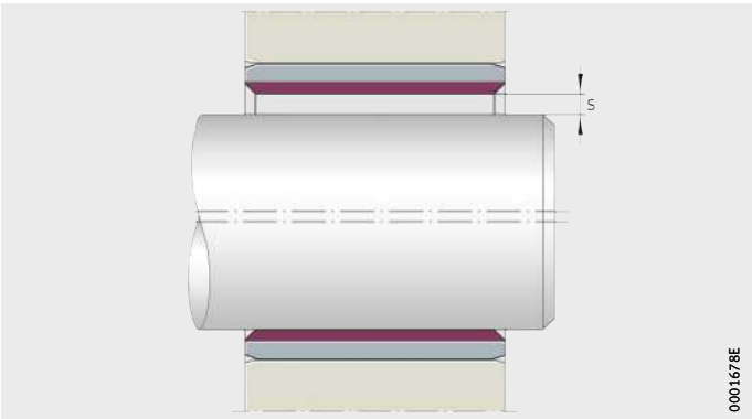
Figure 7 Operating clearance
