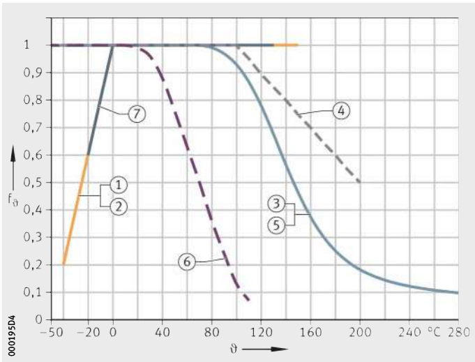
Figure 18 Correction factor for temperature for maintenance-free and low-maintenance bearings
