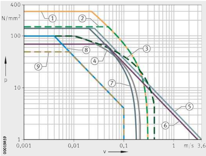
Figure 2 pv diagram
