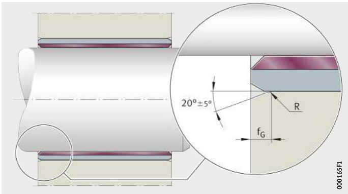
Figure 5 Chamfer on housing bore
