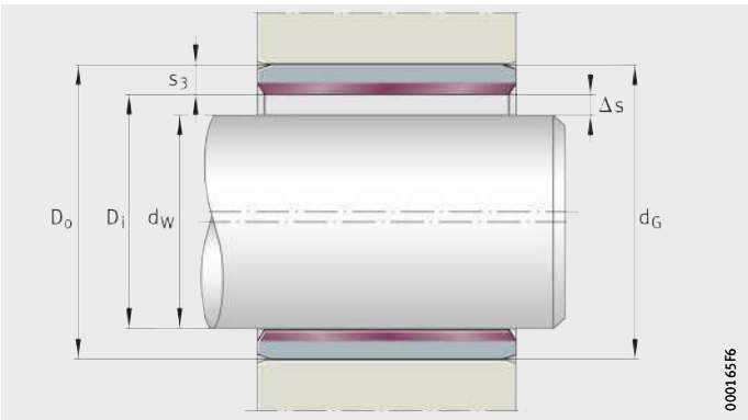
Figure 6 Theoretical bearing clearance
