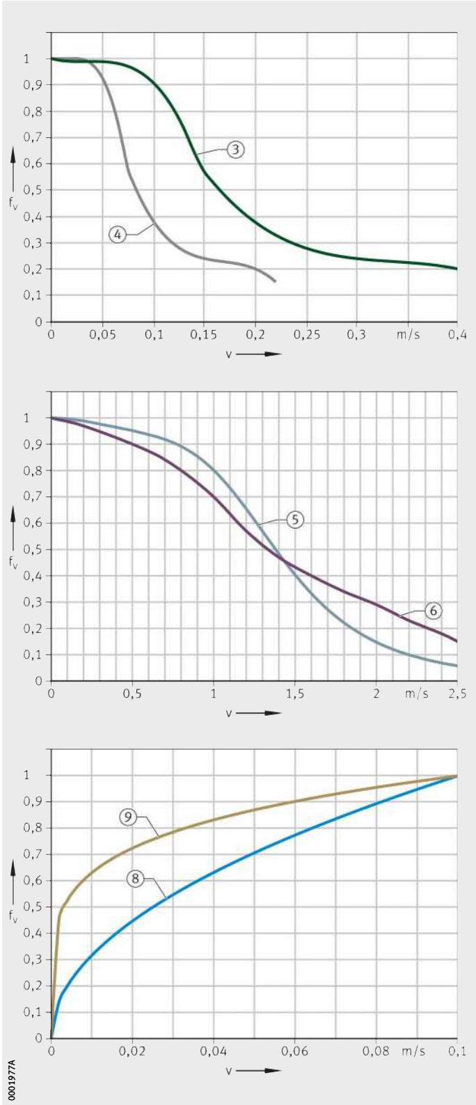
f_v = correction factor v = sliding velocity, see page 44 ③ PTFE composite ④ PTFE film ⑤ E40 ⑥ E50 ⑧ Steel/steel ⑨ Steel/bronze Figure 16 Correction factor for sliding velocity
