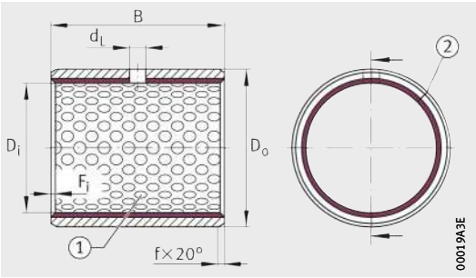
EGB ① Lubrication pockets, ② Butt joint
